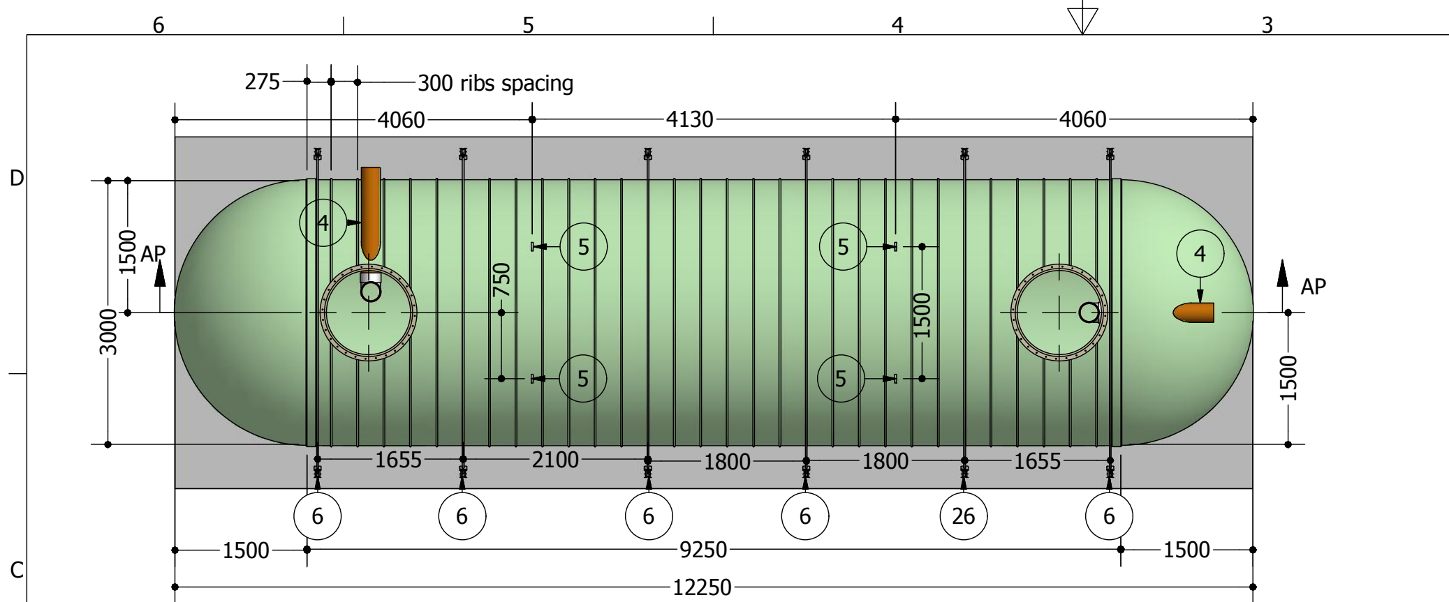
TOP VIEW SCALE 1 / 60
